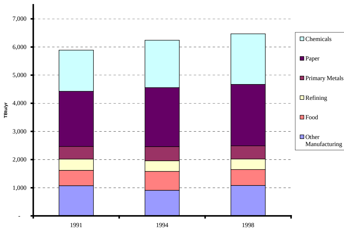
Figure 4-4 MECS Fuel for Boilers 1991-1998
