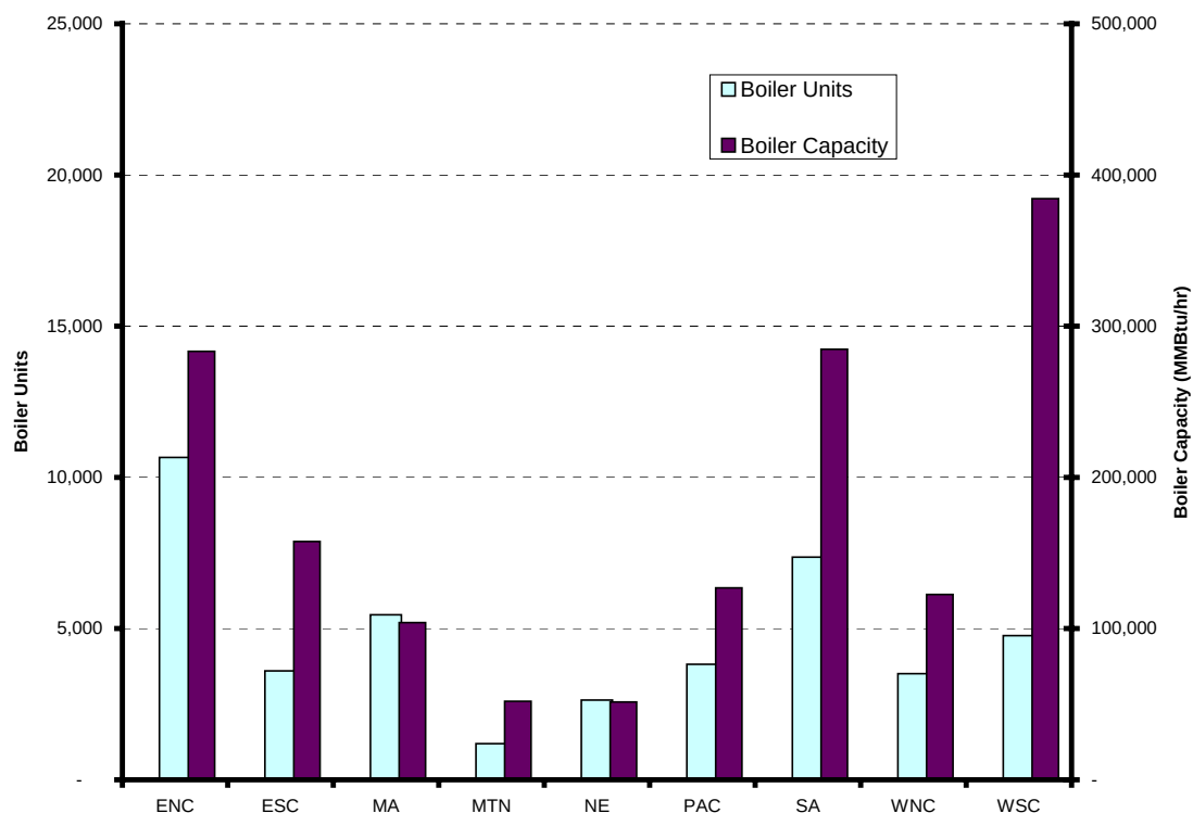
Figure 2-4 Industrial Boilers and Boiler Capacity by Region
