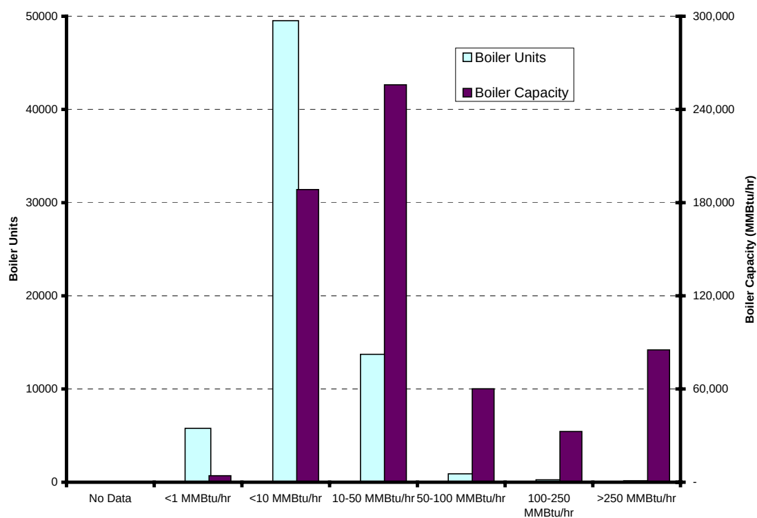
Figure A-1 Size Distribution of Boilers Sold 1992-2002
