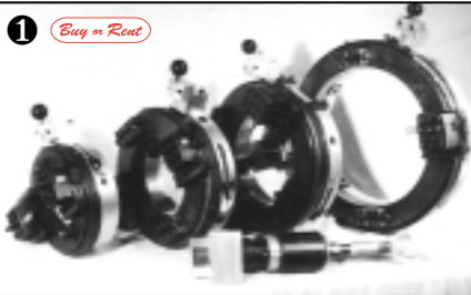
End Prep Lathes and Flange Facers 2" - 36" ID mount
