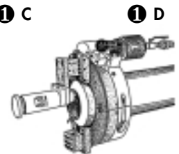
3 Portable Mills Buy or Rent 12" - 96" mills, 6" - 66" travel
