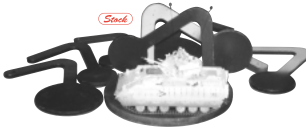
5 Paddle Blinds Buy or Rent 516 grade 70 material Ground edges, drilled, stamped with line size and pound rating, painted.
