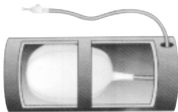
10 Cylinder-Bag Plug
