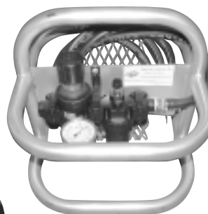
9 Air Filter Regulation Lubricator for pneumatic wrench
