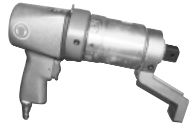
3 Pneumatic Wrench Speed torque wrench. Air driven torque multiplier.
